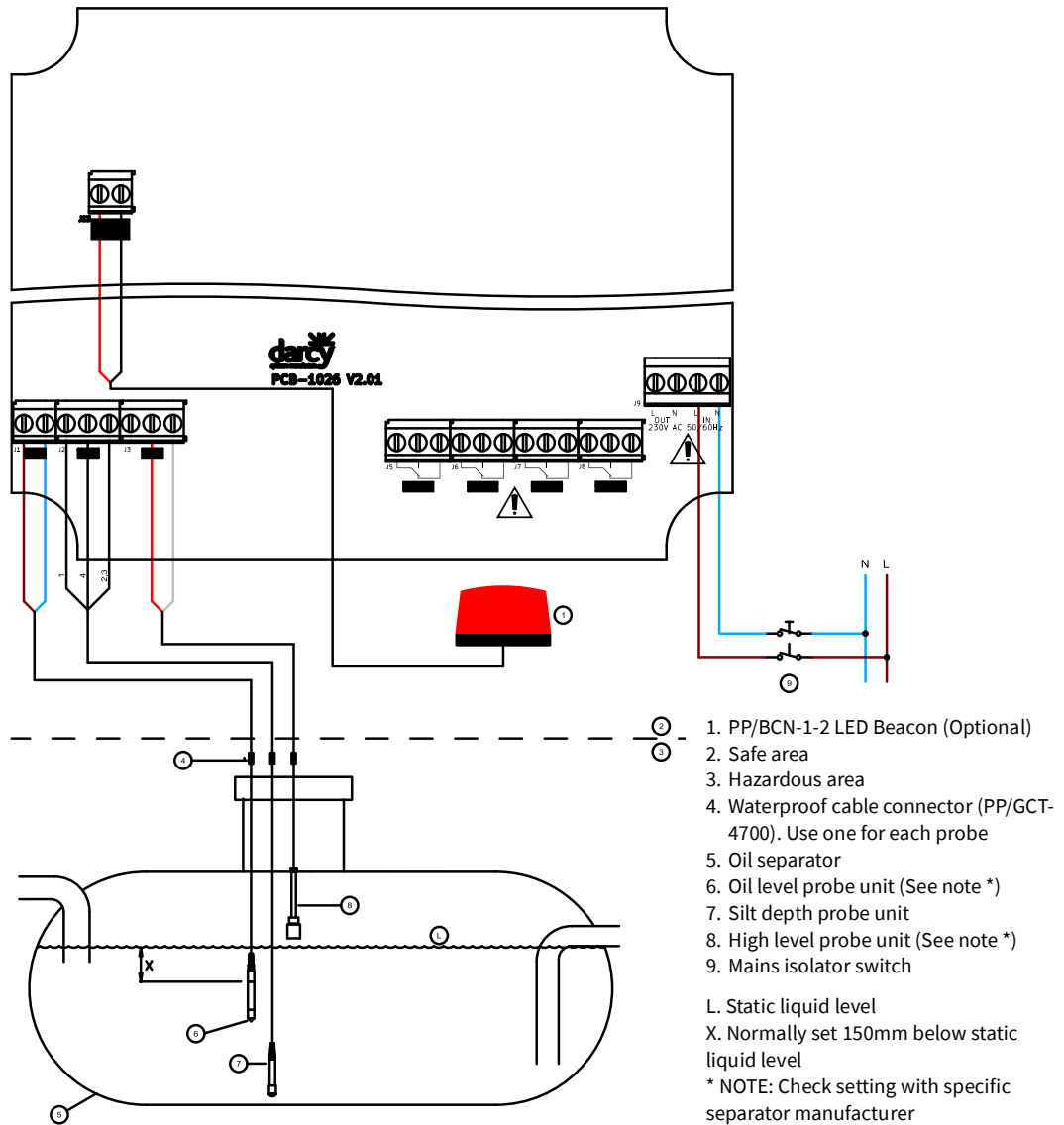
Figure 2: Typical installation for an oil separator alarm: Wiring probes, beacon and mains supply
