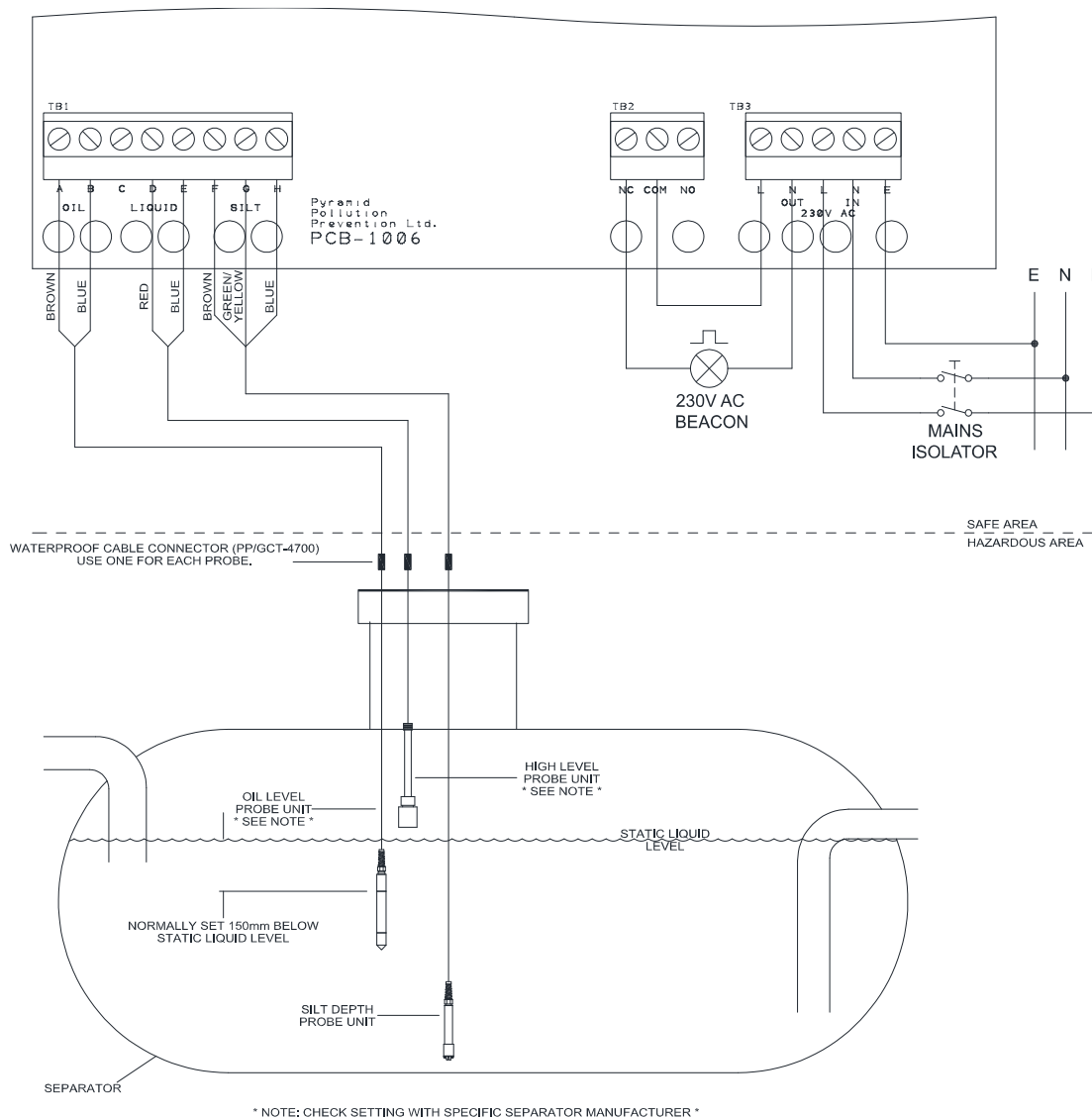
Figure 3 - 14300 separator alarm installation
