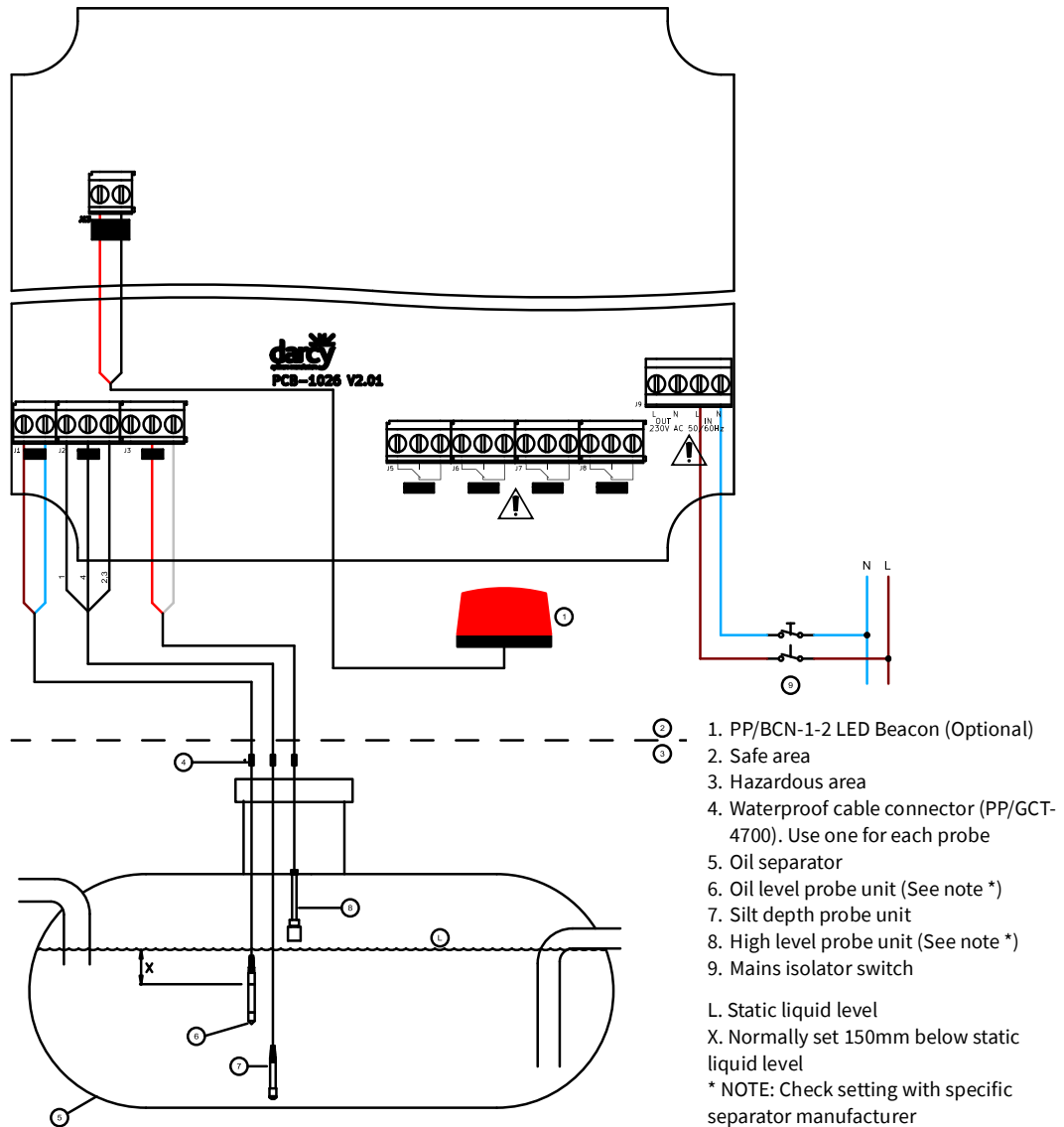
Figure 2: Oil separator alarm installation: Wiring probes, beacon and mains supply
