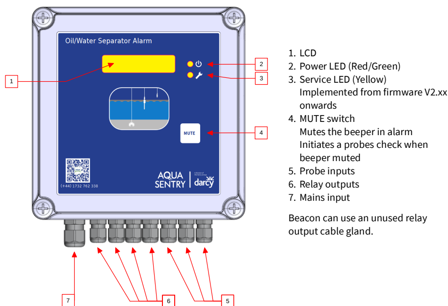
Figure 1: Cable glands, LCD and push button positions
